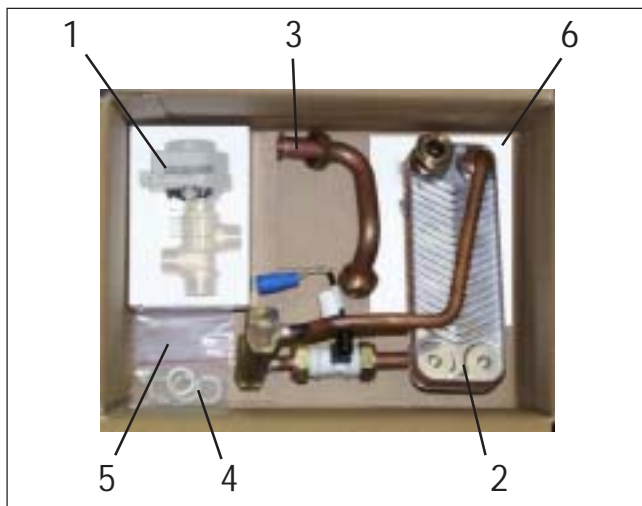
Fig. 1: Conversion set contents
